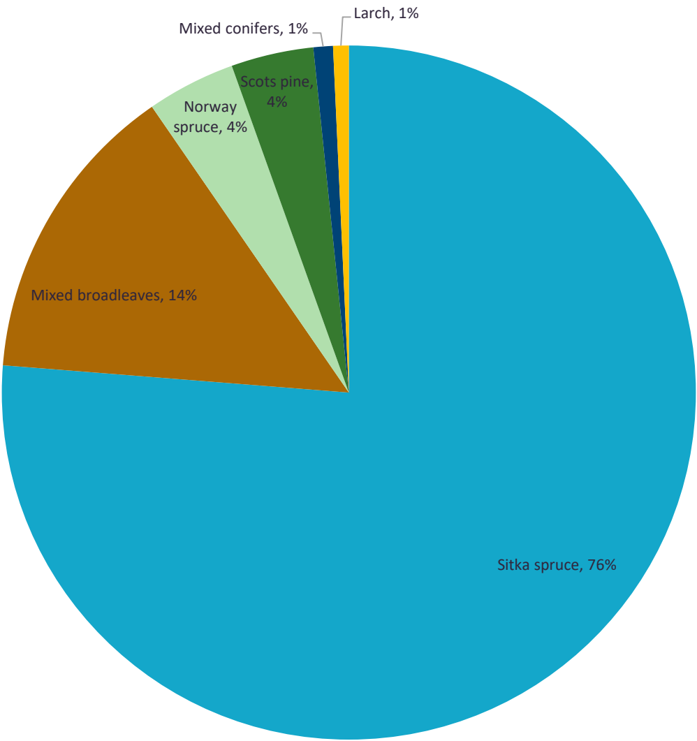
Proportion of forest by species (%)
