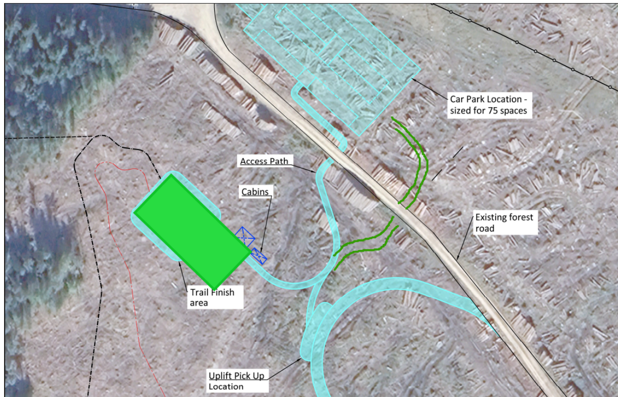
Map showing layout of car park, finish area and uplift pick-up point
